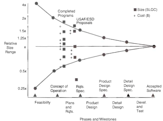
Figure 1: The Cone of Uncertainty [2]
